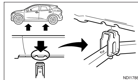
Jacking points
