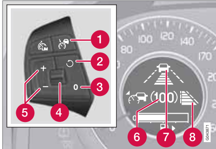
Steering wheel keypad 3 and display.
