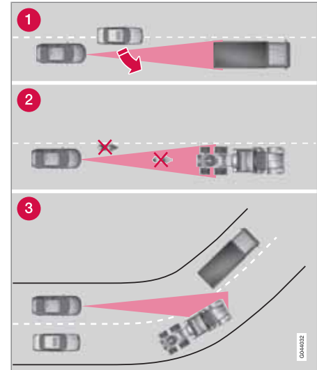
ACC field of vision.
