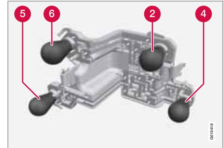
Rear lamp bulb holder
