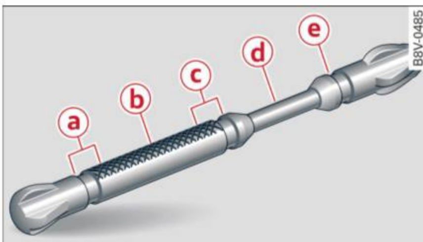
Fig. 160 Diesel engine oil dipstick: guide for measuring the oil level (example)
