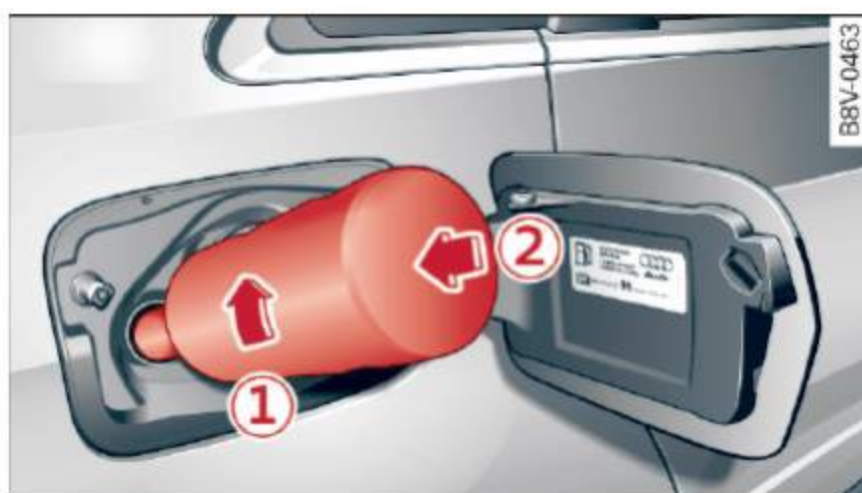
Fig. 154 AdBlue filler tube: inserting the refill bottle
