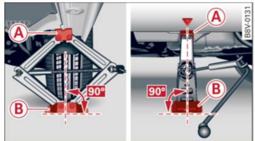
Fig. 179 Sill: positioning the vehicle jack
