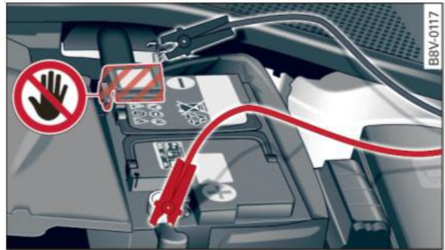
Fig. 164 Engine compartment: connectors for a charger and jump start cables
