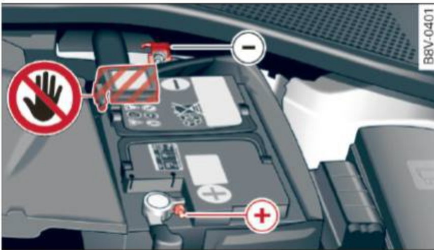
Fig. 188 Engine compartment: connectors for jump start cables and a charger
