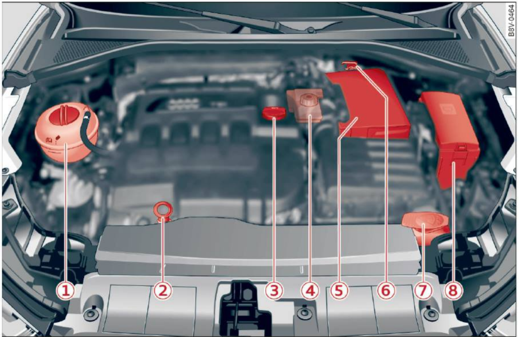
Fig. 158 Typical location of the reservoir, engine oil dipstick, and engine oil filler opening
