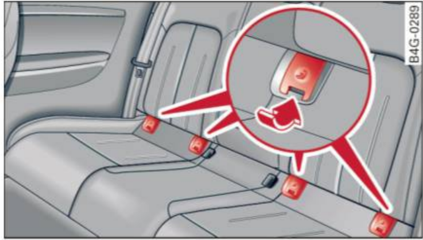
Fig. 144 Lower anchorages, covers marked
