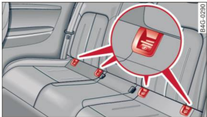
Fig. 145 Rear seats: lower anchorage bracket locations
