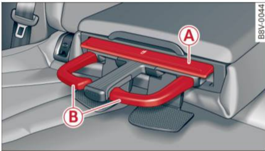
Fig. 53 Section of the rear bench seat: rear cup holders*
