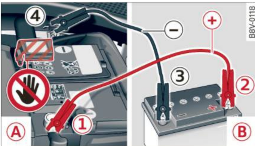
Fig. 189 Jump starting the battery with another vehicle: (A) - drained battery, (B) - starter battery
