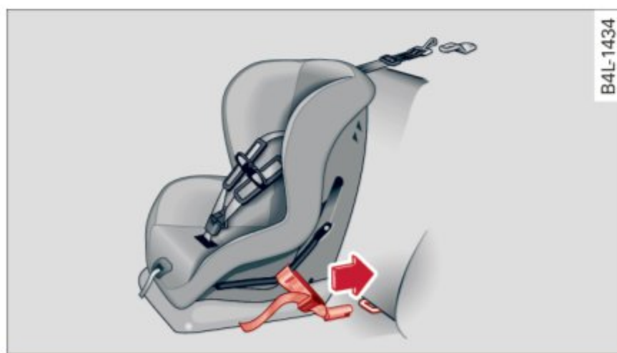
Fig. 146 Lower anchorages: proper mounting
