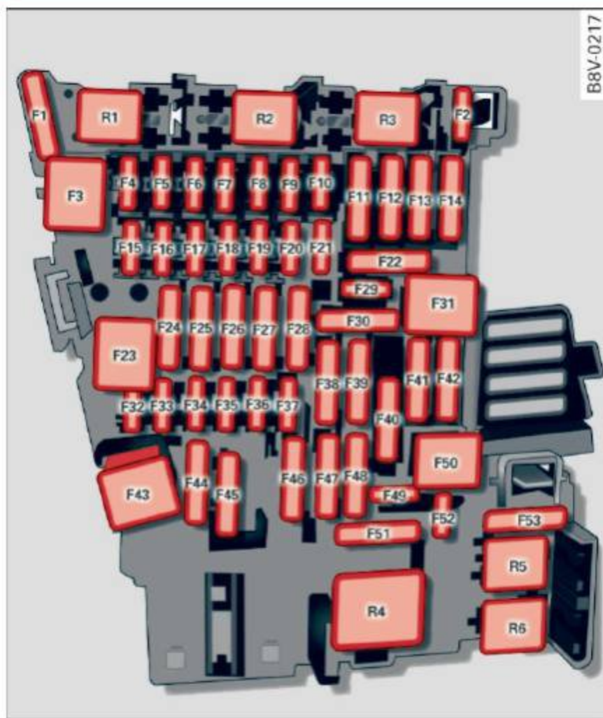
Fig. 186 Vehicle interior: fuse assignment
