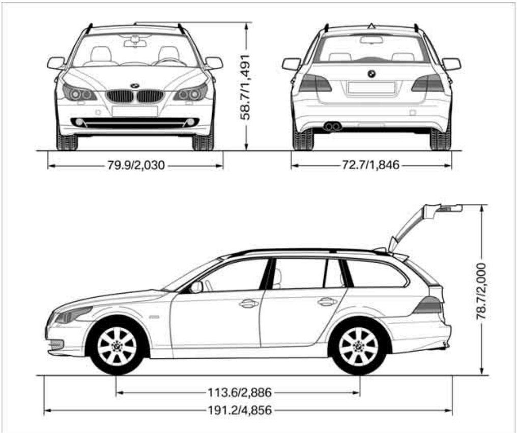
All dimensions given in inches/mm. Smallest turning circle diam.: 39 ft/11.9 m
