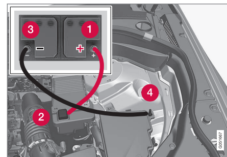
Jumper cable connecting points. Engine compartment appearance may vary depending on vehicle model and equipment level.
