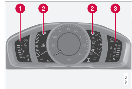
Indicator and warning symbols: analog instrument panel
