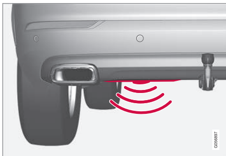
The foot movement sensor is located to the left of center under the rear bumper 6
