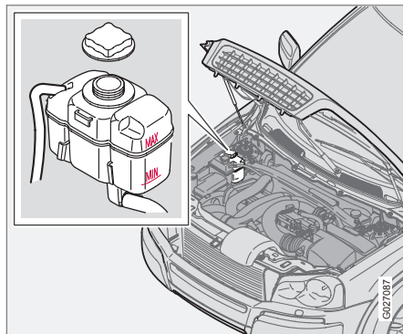
Coolant reservoir
