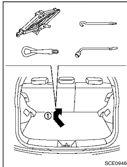
Jacking tools
